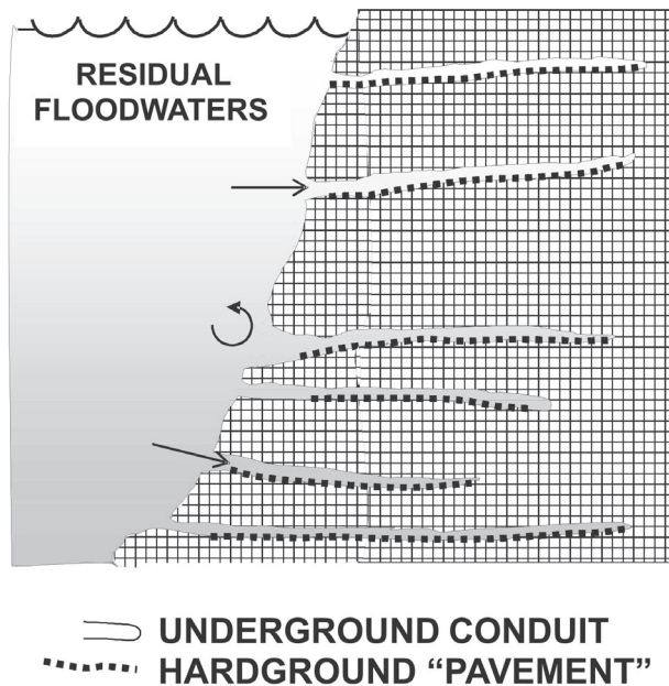
Figure 2. The conduit-hardground hypothesis. Horizontal conduits form in previously lithified Flood-deposited strata. Thanks to episodic forced movements of water, hardgrounds of varying complexity form on the floors of these flat submarine cavelike conduits. Note the potential ability of multiple horizons of hardgrounds to form long after the Flood itself and the extreme vertical exaggeration in this figure.
