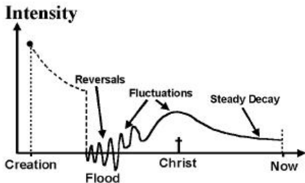
Magnetic field intensity at the earth's surface
