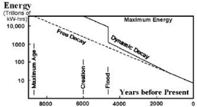
Energy stored in the Earth's magnetic field
